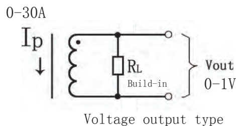
Schematic Diagram
